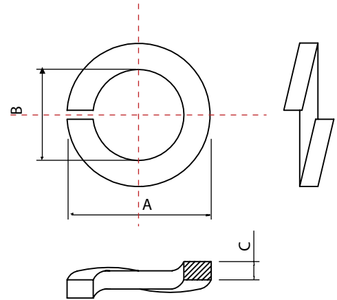
ARANDELA GROWER
